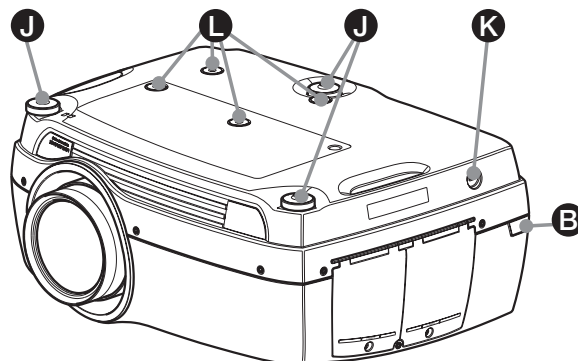
Figure 4-3. - Projector bottom view
