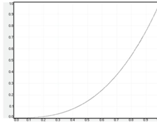
Figure 7-2. Film 2.8 gamma
