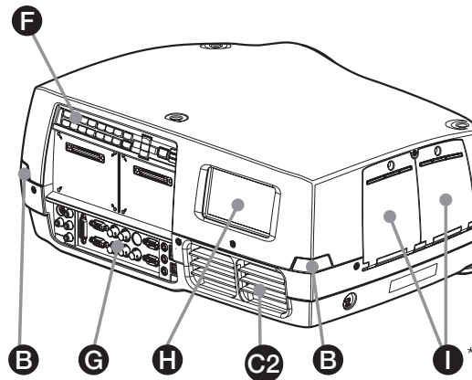
Figure 4-2. - Projector rear view
